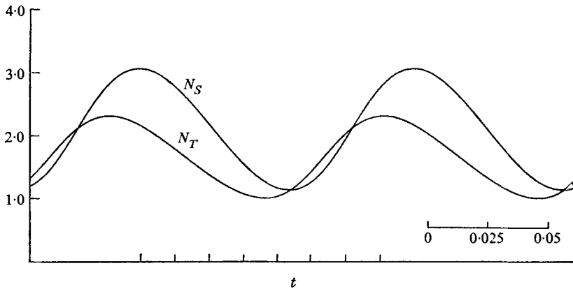
FIGURE 6. The thermal and saline Nusselt numbers as a function of time for R_1 < R_T = 8600 < R_2 , R_S = 10^4 , \sigma = 1 and \tau = 10^{-1} . The marks on the time axis indicate the times at which the stream function, temperature, salinity and density fields are displayed in figure 8. The horizontal line in the bottom right-hand corner represents 0.05 non-dimensional time units.
