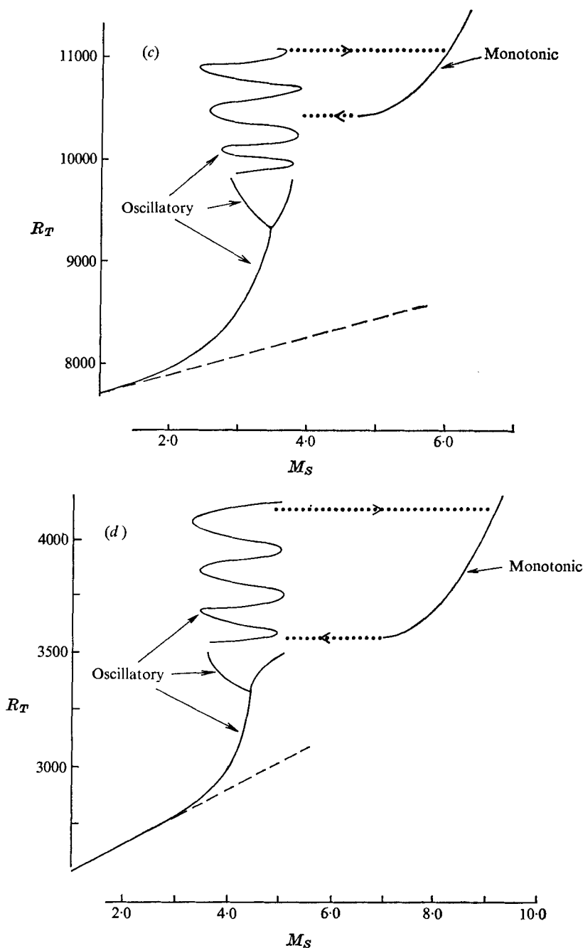
FIGURE 5. The stable solution branches in an R_T, M_S plane for (a) \sigma = 1, \tau = 10^{-4}, R_S = 10^3 , (b) \sigma = 1, \tau = 10^{-4}, R_S = 10^4 , (c) \sigma = 1, \tau = 10^{-4}, R_S = 10^4 and (d) \sigma = 1, \tau = 0.1, R_S = 10^4 . For R_3 < R_T < R_4 both local maxima are shown and for R_3 < R_T < R_4 the rapidly oscillating curve indicates that no definite maximum can be assigned to the aperiodic motion in this range. The dots indicate the transitions that can take place between the oscillatory and monotonic branches. The dashed curve is the first approximation to the oscillatory solution branch, as obtained from (4.7).
