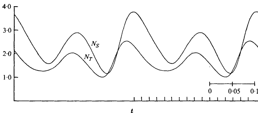
FIGURE 9. The thermal and saline Nusselt numbers as a function of time for
