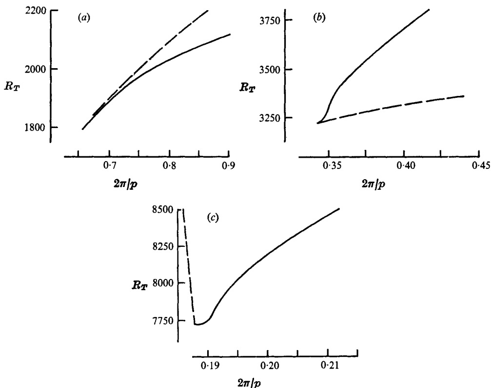
FIGURE 4. The period of oscillation 2\pi/p as a function of R_T for \sigma = 1 , \tau = 10^{-4} and (a) R_S = 10^3 ( R_1 = 1797 ), (b) R_S = 10^4 ( R_1 = 3220 ) and (c) R_S = 10^4 ( R_1 = 7720 ). —, result obtained from the numerical calculation of \mathcal{S} ; ---, result obtained from the modified perturbation expansion of § 4.
